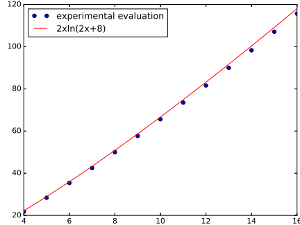
Figure 3: Average Stopping Time Approximation
