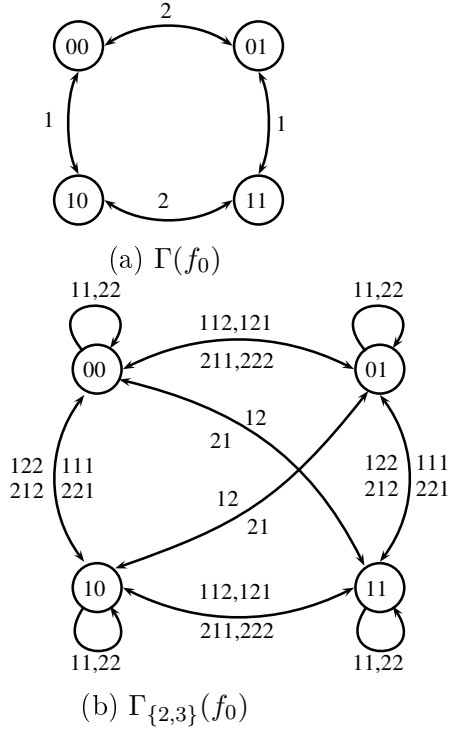
Figure 2: Iterating f_0 : (x_1, x_2) \mapsto (\bar{x}_1, \bar{x}_2)
