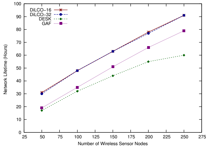
Figure 25: The Network Lifetime for Lifetime50
