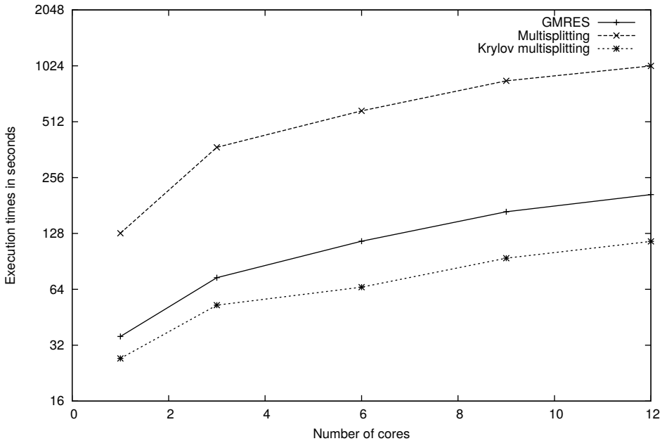
Execution times in seconds for each method
