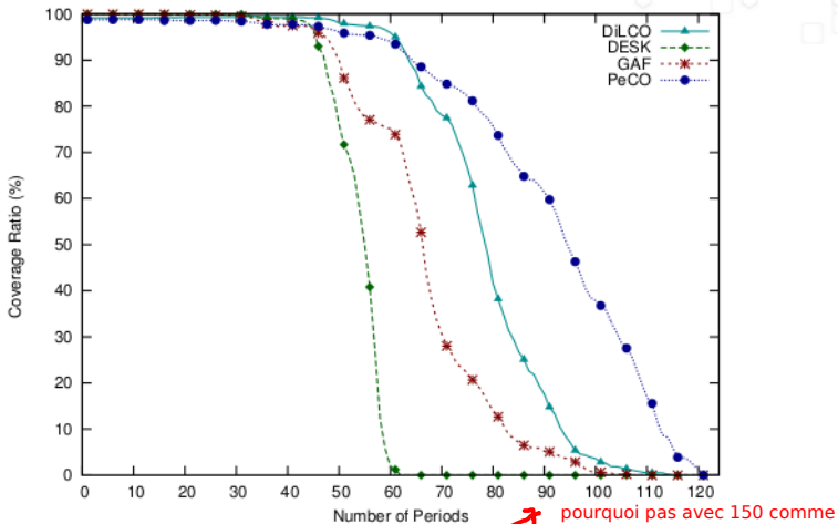
FIGURE: Coverage ratio for 200 deployed nodes.
