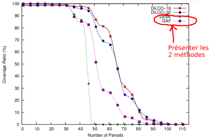
FIGURE: Coverage ratio for 150 deployed nodes
