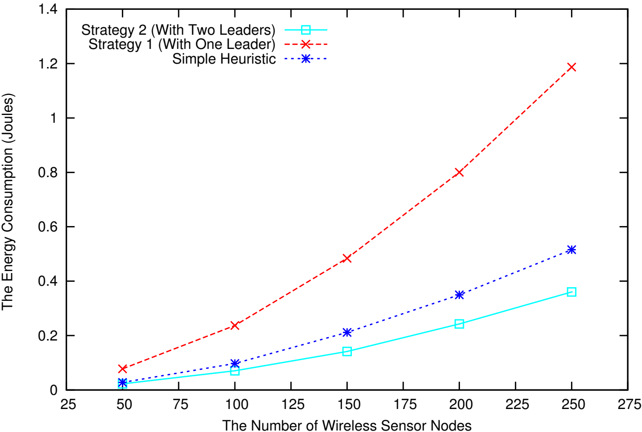
The Energy Consumption (Joules) vs The Number of Wireless Sensor Nodes
