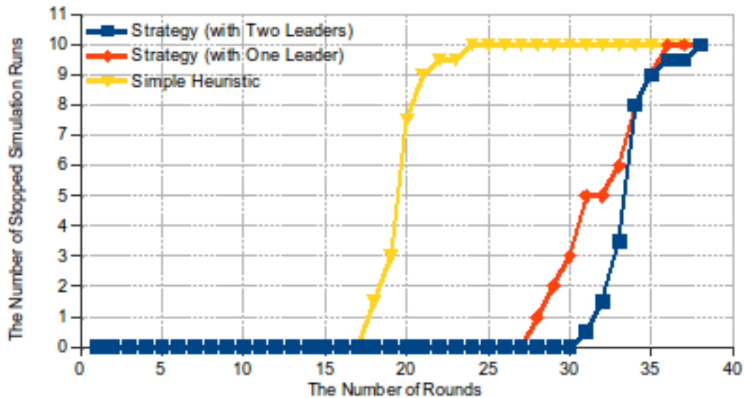
The Number of Stopped Simulation Runs vs The Number of Rounds
