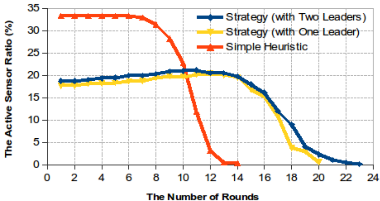
The Active Sensor Ratio (%) vs The Number of Rounds
