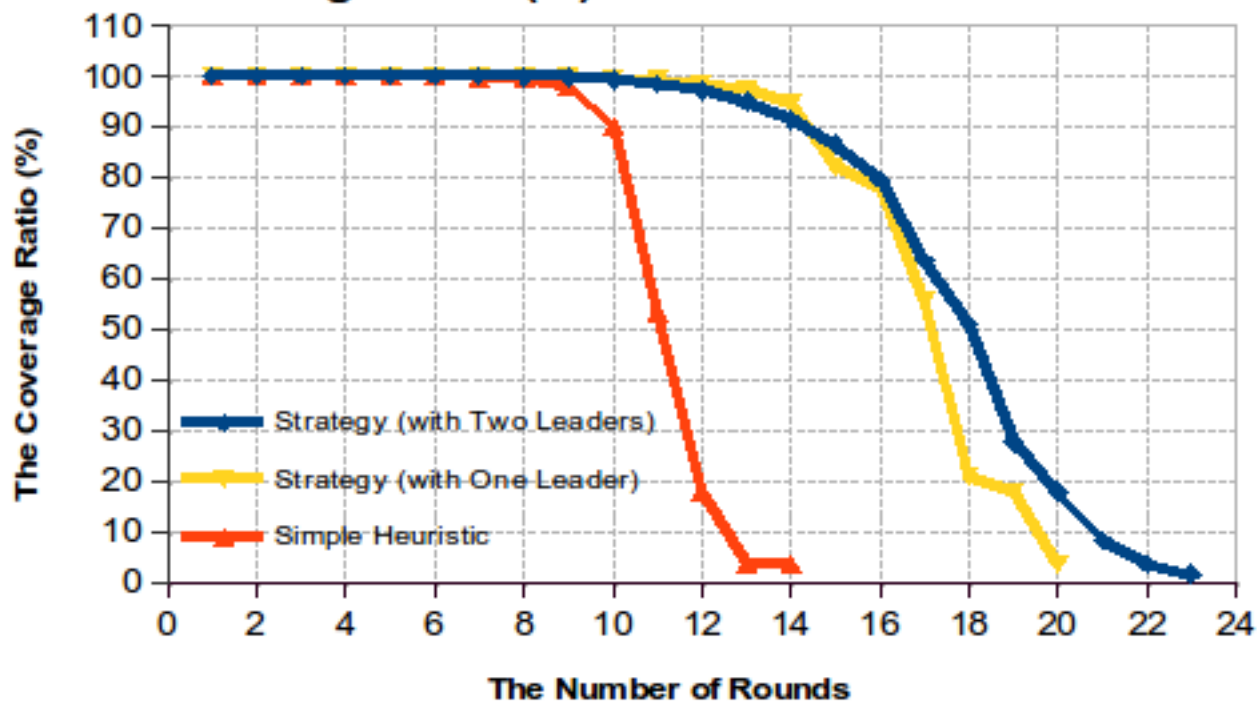
The Coverage Ratio (%) vs The Number of Rounds
