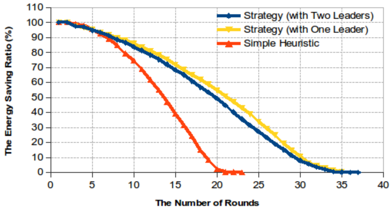
The Energy Saving Ratio (%) vs The Number of Rounds
