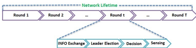
Figure 1: Multi-round coverage protocol
