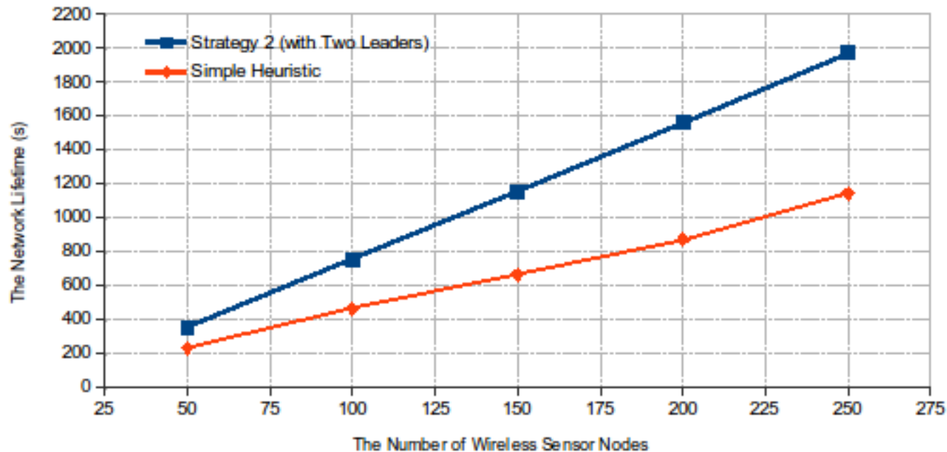
The Network Lifetime (s) vs The Number of Wireless Sensor Nodes
