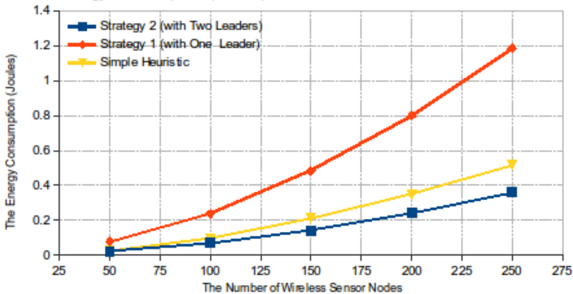
The Energy Consumption (Joules) vs The Number of Wireless Sensor Nodes
