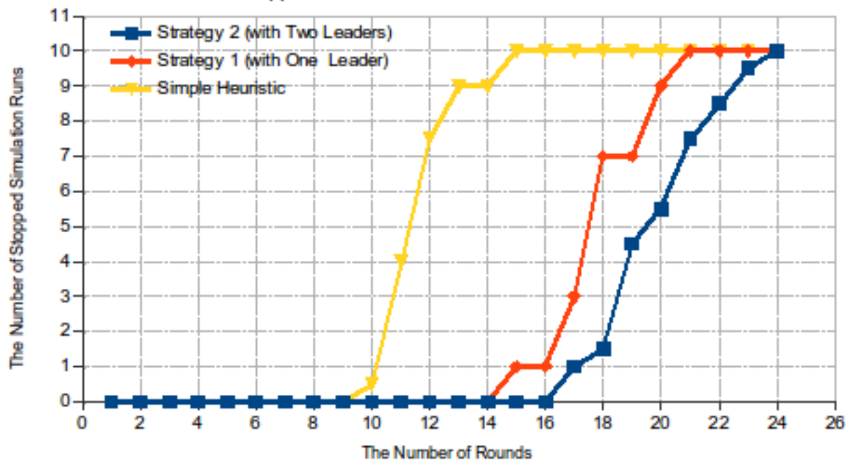
The Number of Stopped Simulation Runs vs The Number of Rounds
