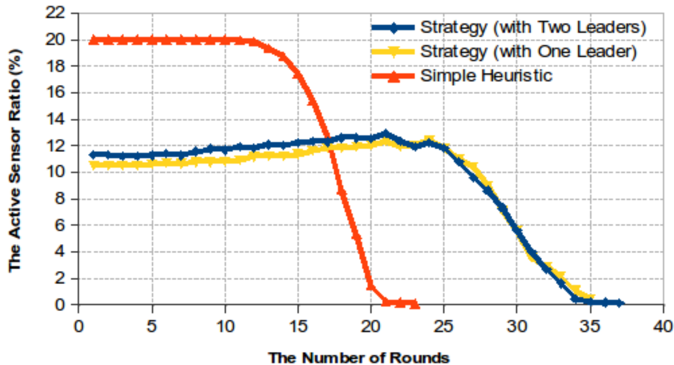
The Active Sensor Ratio (%) vs The Number of Rounds
