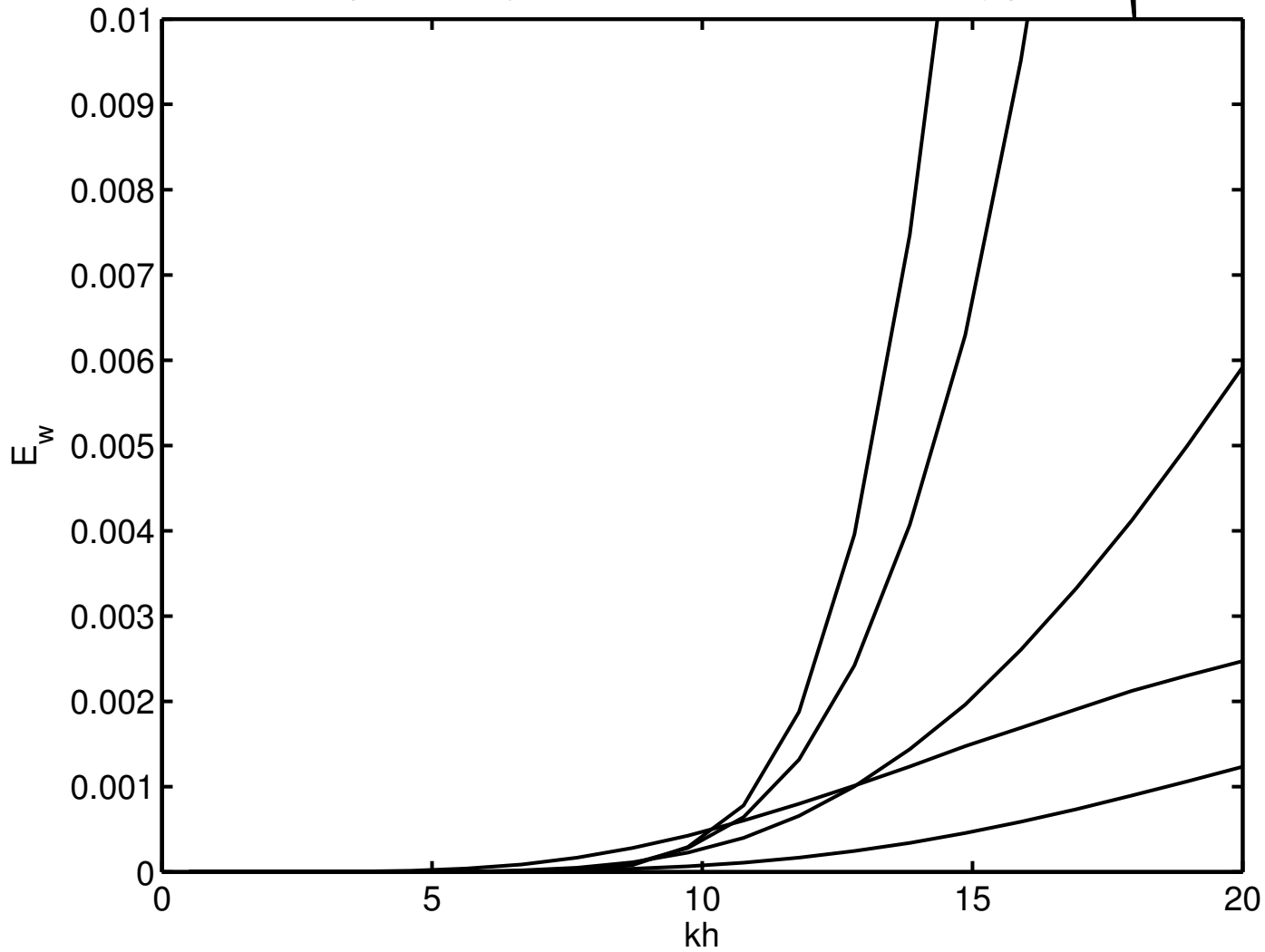
Depth-averaged errors on the vertical velocity profile
