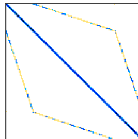
FEM_3D_thermal2
