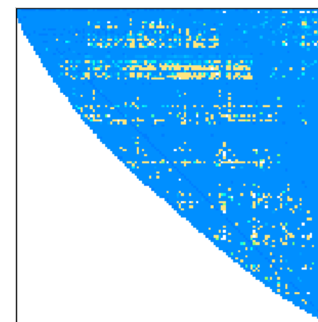
language
