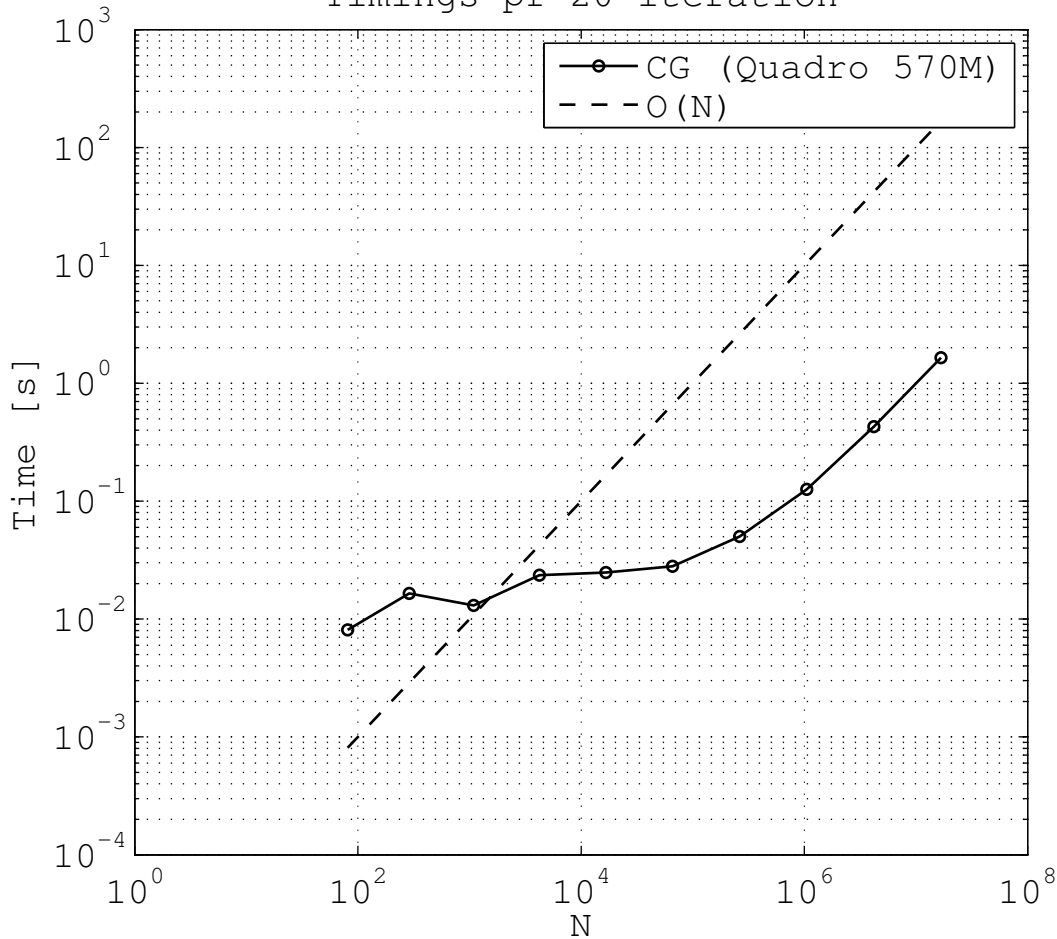
Timings pr 20 iteration
