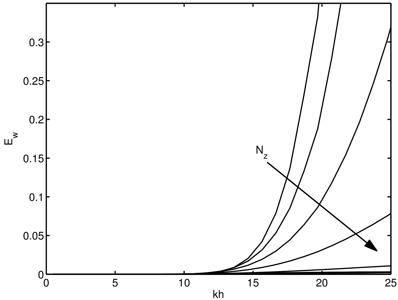
Depth-averaged errors on the vertical velocity profile
