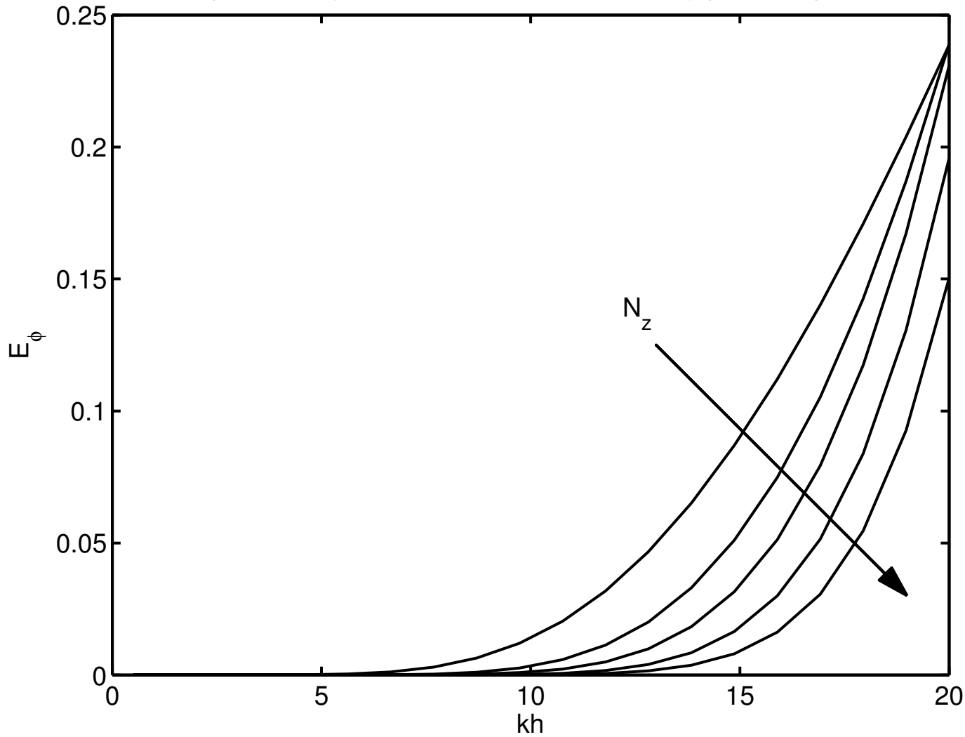
Depth-averaged errors on the scalar velocity potential profile
