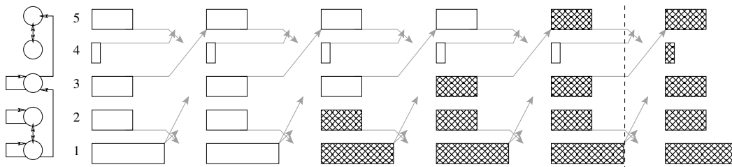
FIGURE 1.5 – Itérations synchrones
