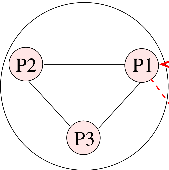
Cluster 3
