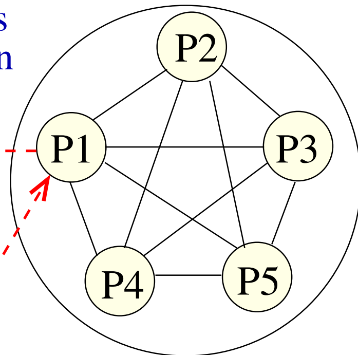
Cluster 2
