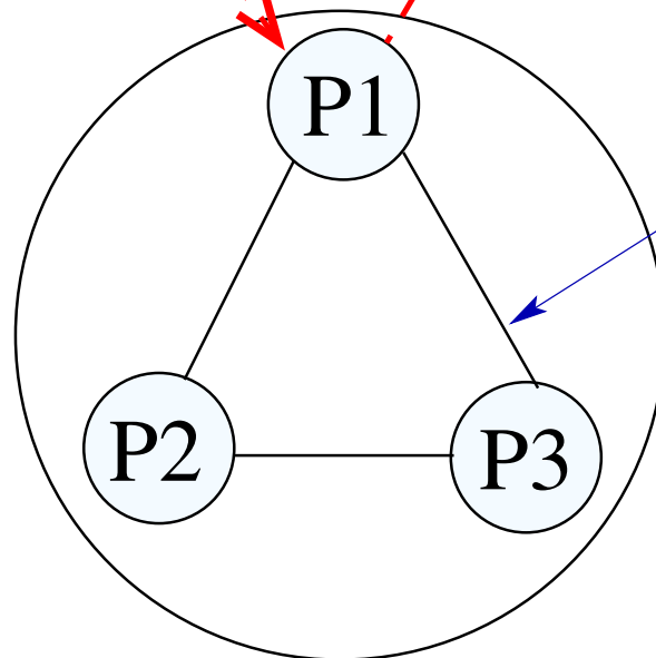
Cluster 1
