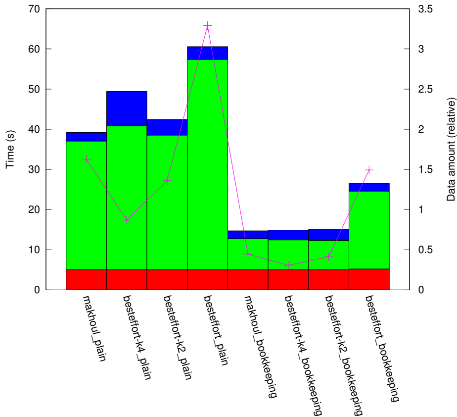
results_IN_1:1/plat_cluster16/topo_hcube
