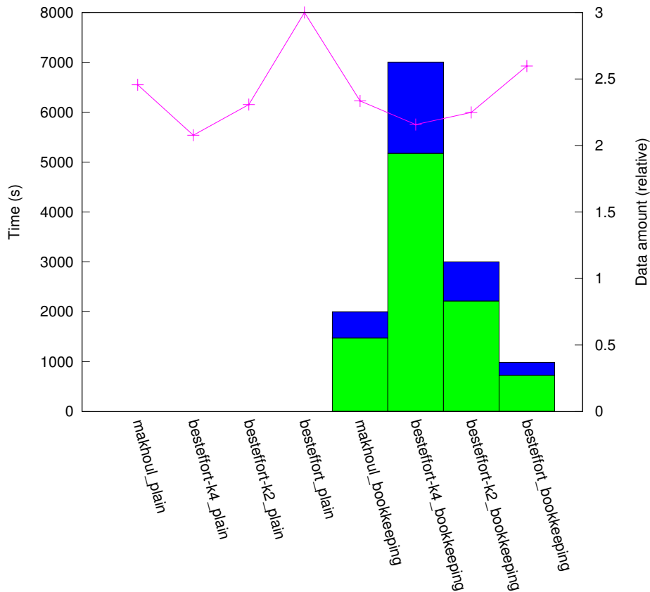
results_IN_1:1/plat_grid64/topo_line
