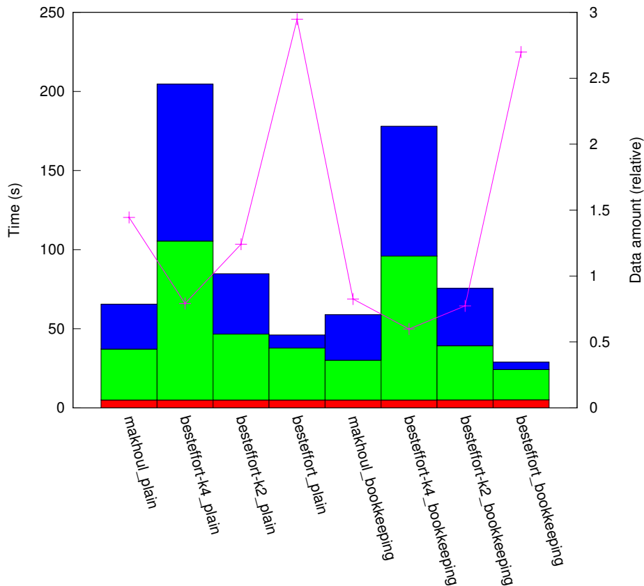
results_IN_10:1/plat_grid256/topo_torus
