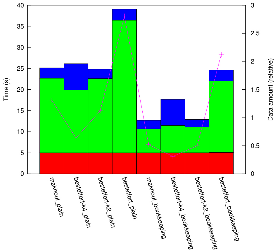
results_IN_10:1/plat_grid16/topo_torus
