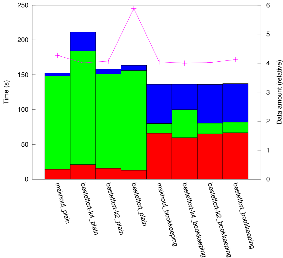
results_l1_1:1/plat_cluster64/topo_torus
