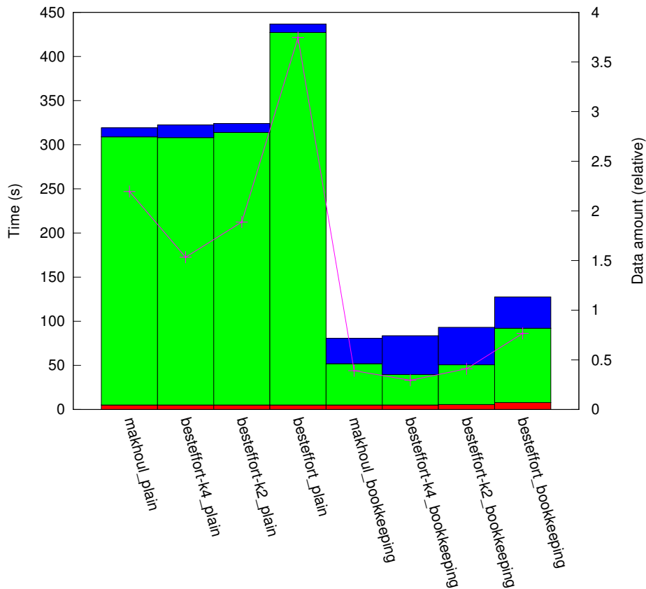
results_IN_1:10/plat_cluster16/topo_torus
