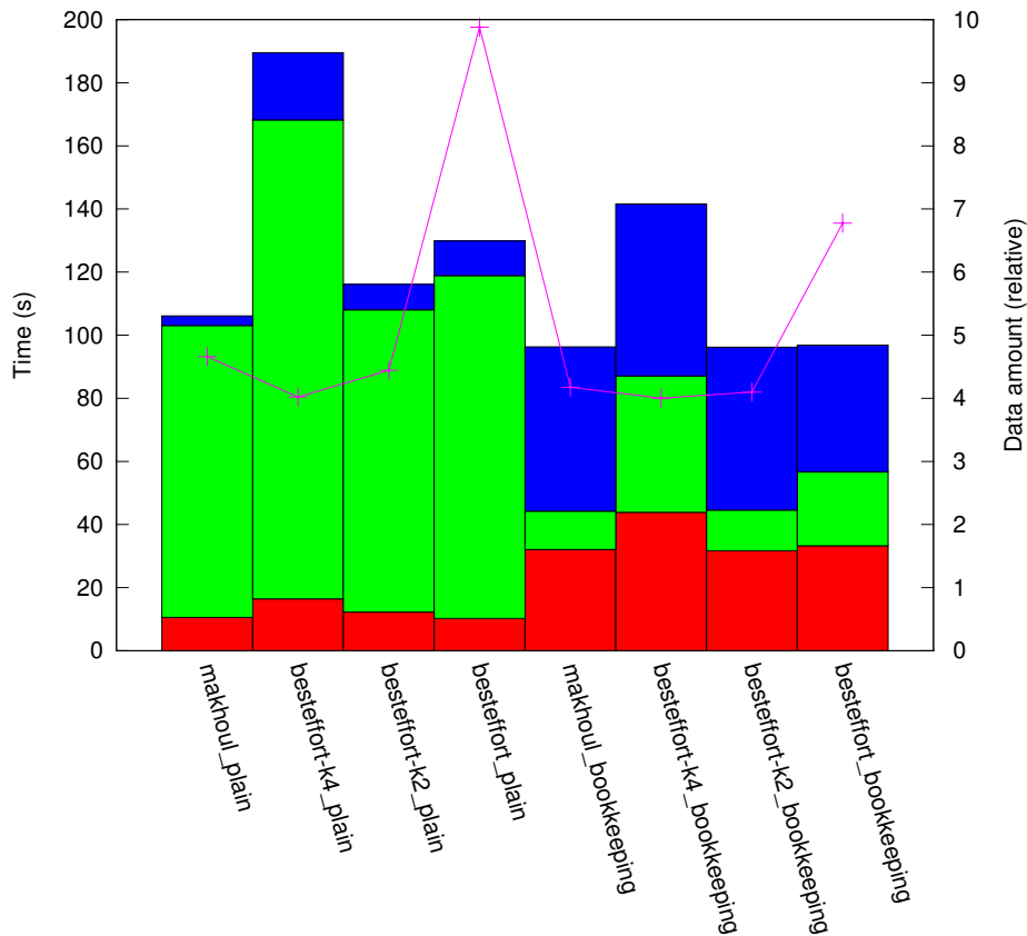
results_I1_10:1/plat_grid256/topo_hcube
