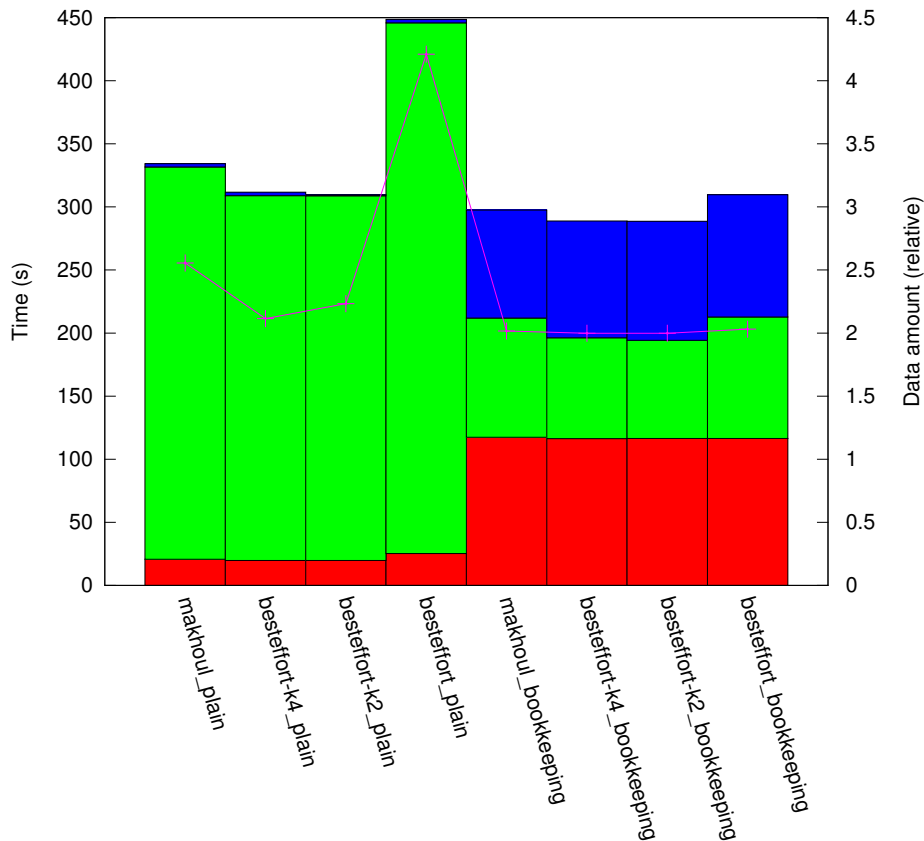
results_I1_1:10/plat_cluster16/topo_hcube
