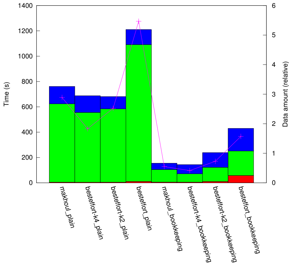
results_IN_1:10/plat_grid256/topo_hcube
