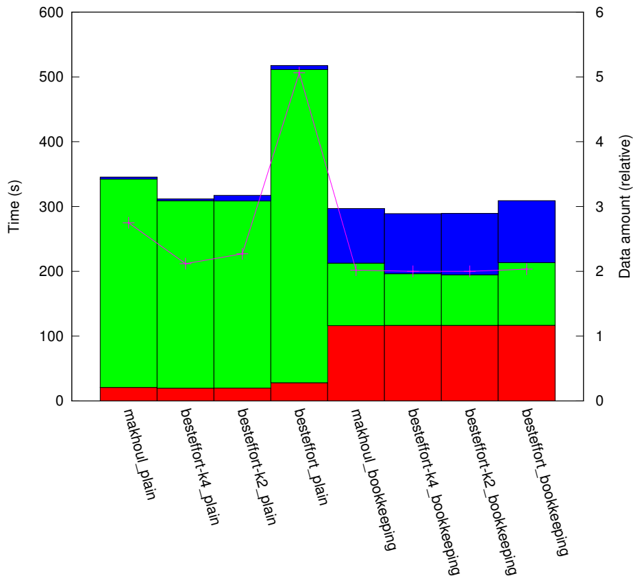
results_R1_1:10/plat_cluster16/topo_torus
