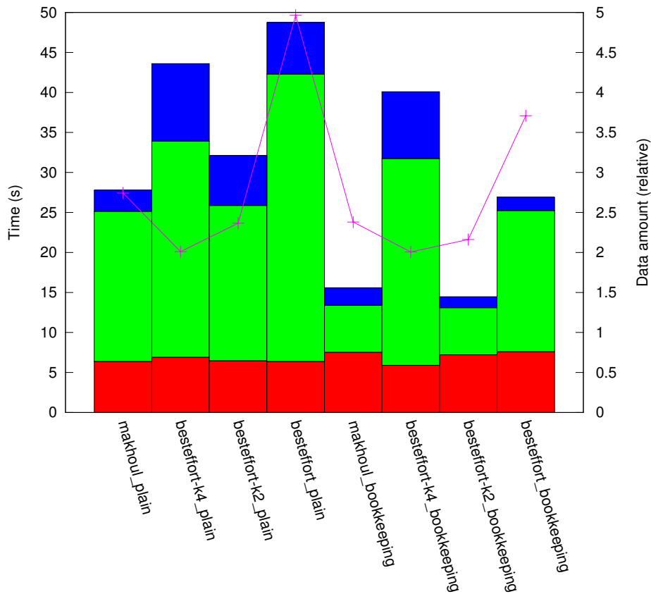
results_R1_10:1/plat_cluster16/topo_torus
