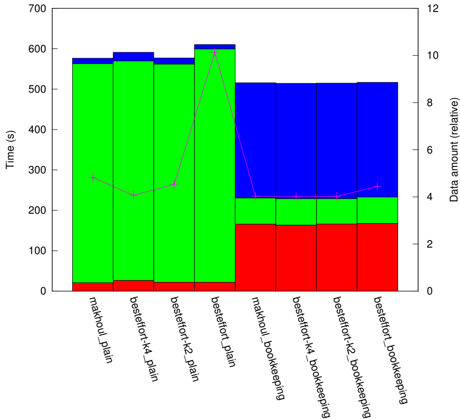
results_R1_1:1/plat_grid256/topo_hcube
