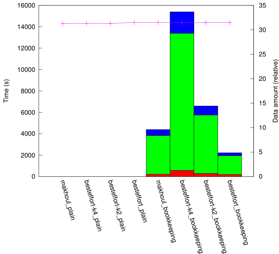
results_l1_1:1/plat_cluster64/topo_line
