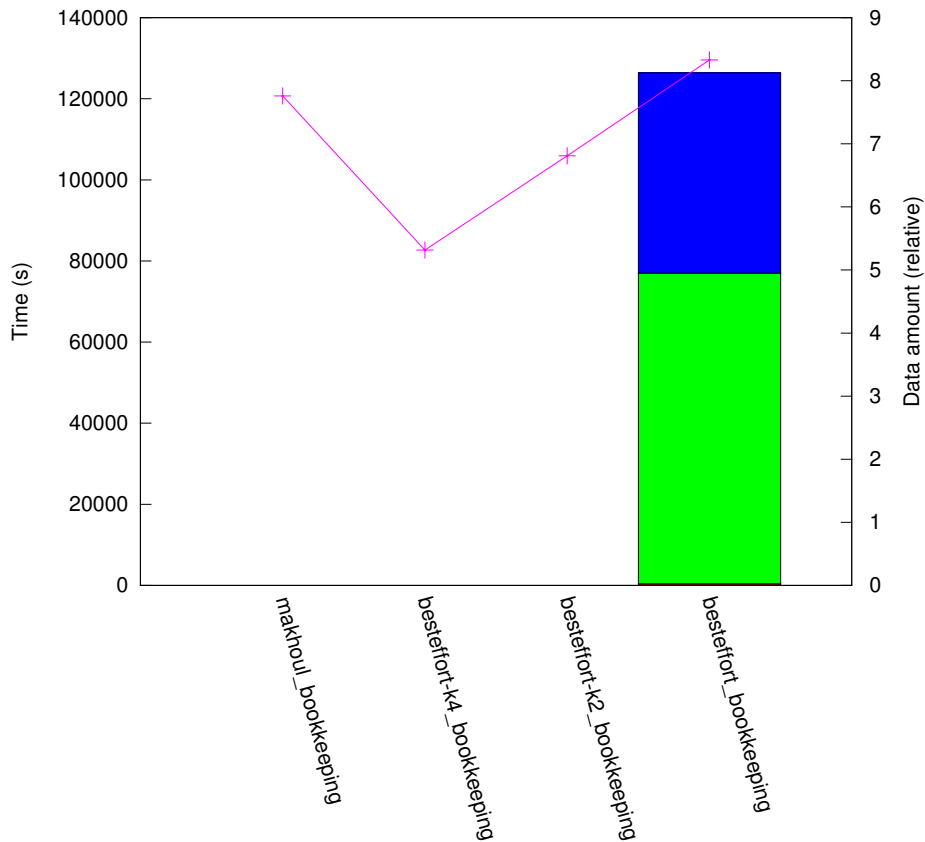
results_IN_1:10/plat_cluster1024/topo_line
