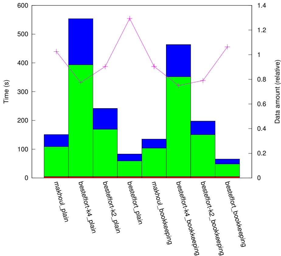
results_IN_10:1/plat_cluster16/topo_line
