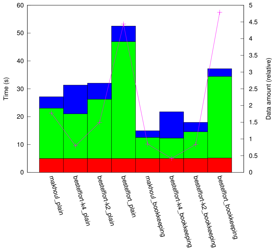
results_IN_10:1/plat_grid64/topo_hcube
