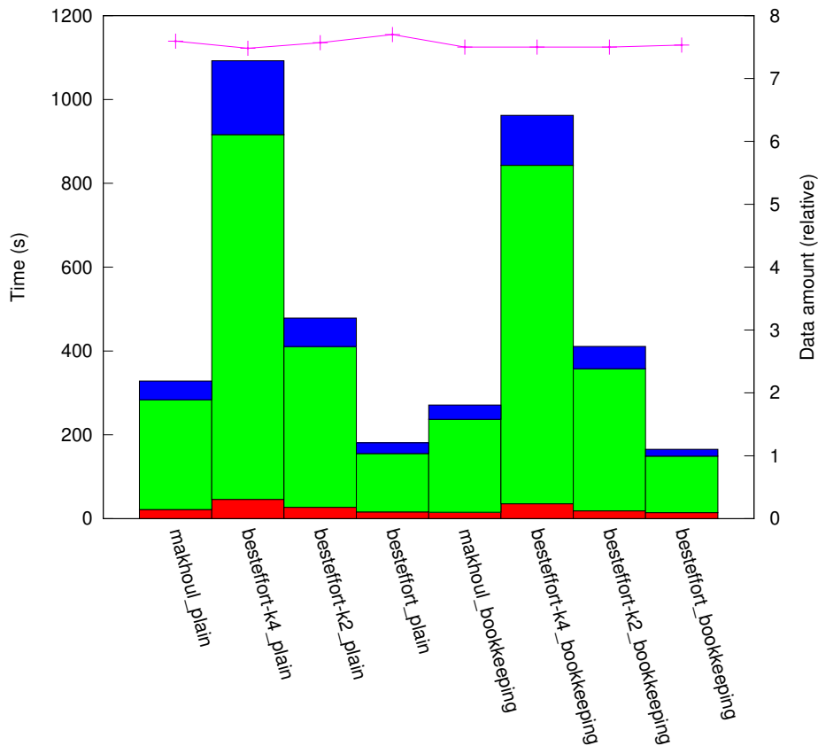
results_I1_10:1/plat_cluster16/topo_line
