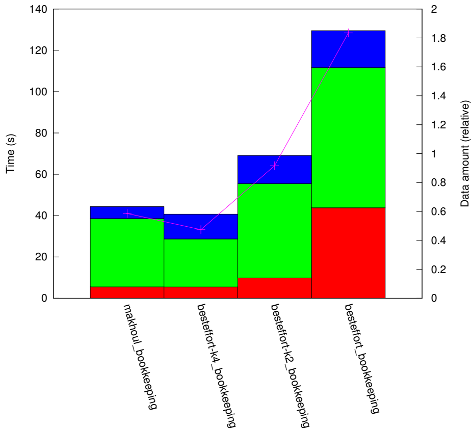
results_IN_1:1/plat_cluster1024/topo_hcube
