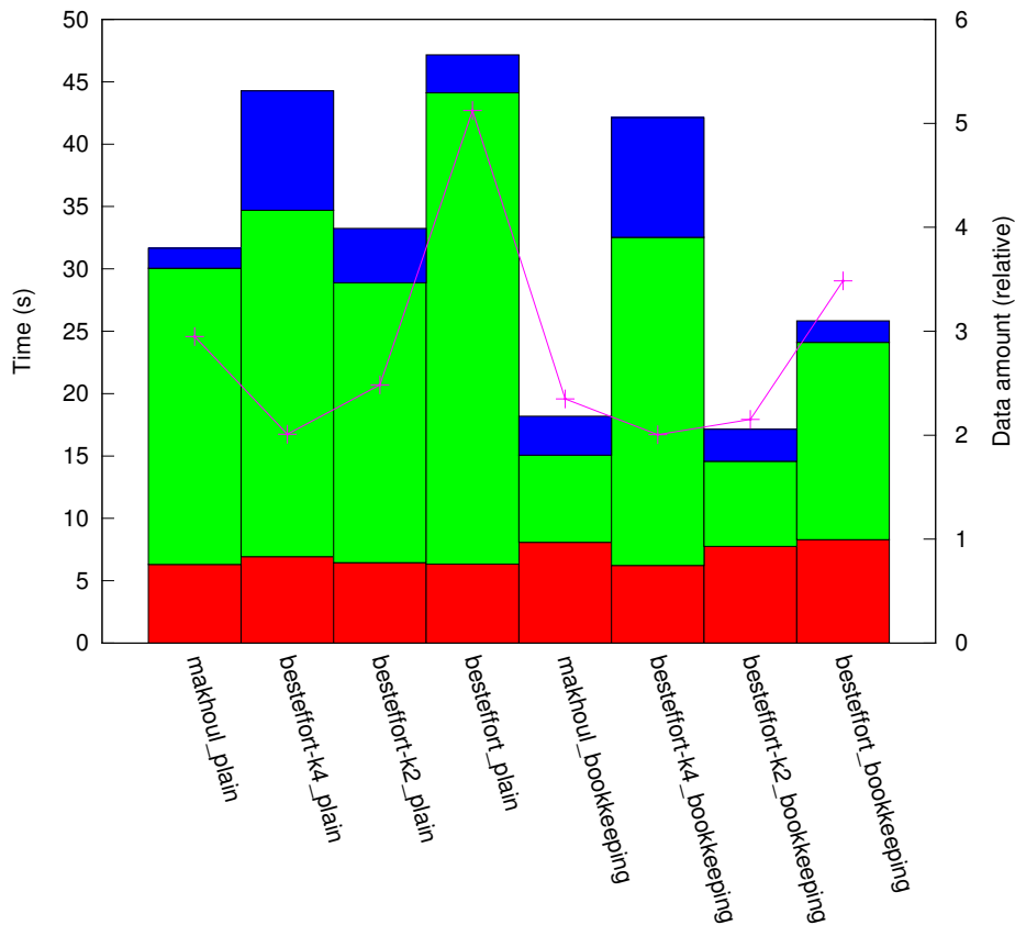
results_I1_10:1/plat_grid16/topo_torus
