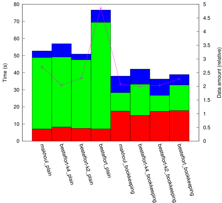
results_I1_1:1/plat_cluster16/topo_hcube
