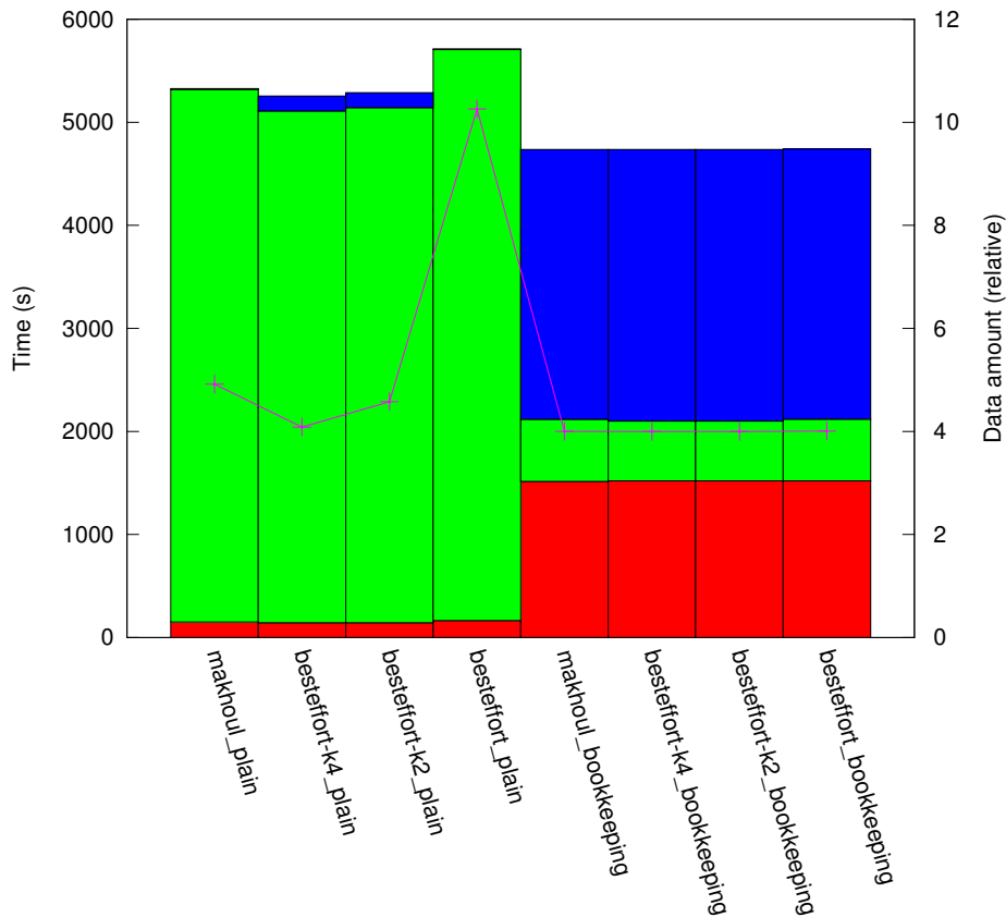
results_R1_1:10/plat_grid256/topo_hcube
