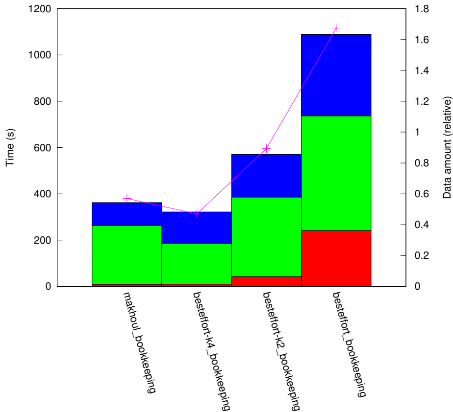
results_IN_1:10/plat_grid1024/topo_hcube
