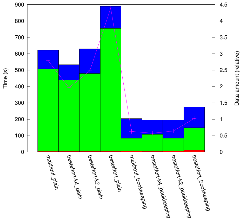
results_IN_1:10/plat_grid256/topo_torus
