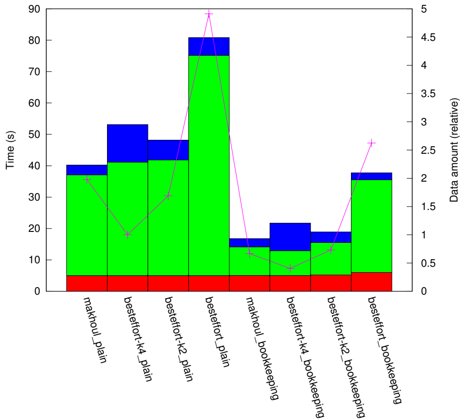
results_IN_1:1/plat_cluster64/topo_hcube
