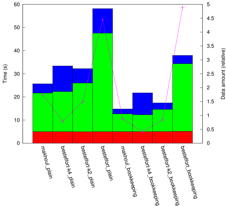
results_IN_10:1/plat_cluster64/topo_hcube
