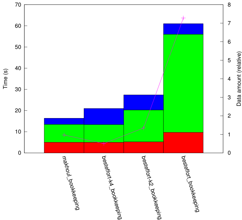
results_IN_10:1/plat_grid1024/topo_hcube
