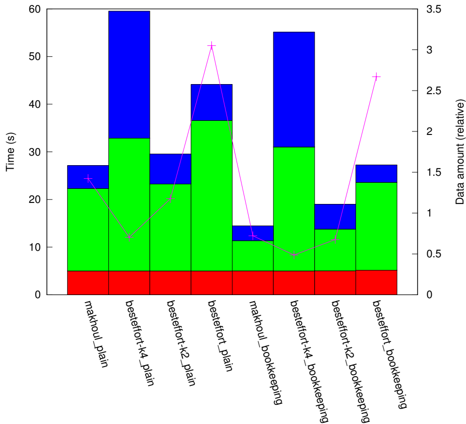
results_IN_10:1/plat_grid64/topo_torus
