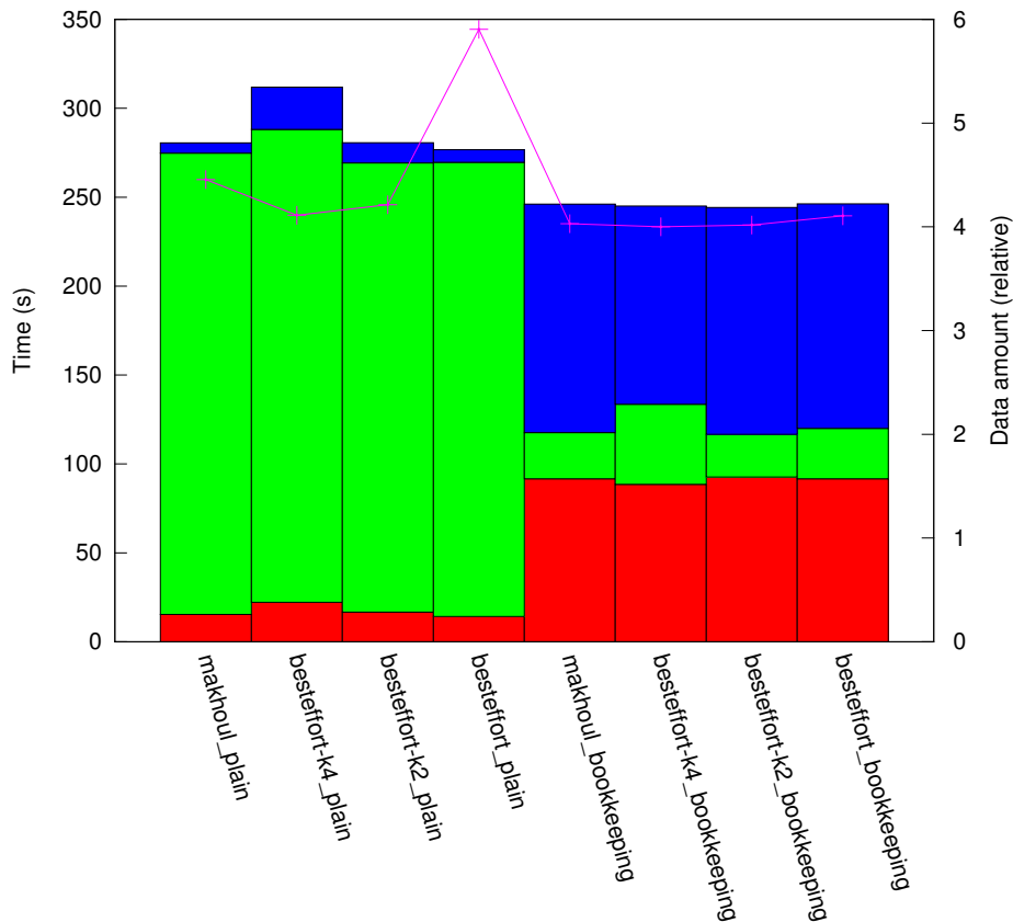
results_l1_1:1/plat_grid64/topo_torus
