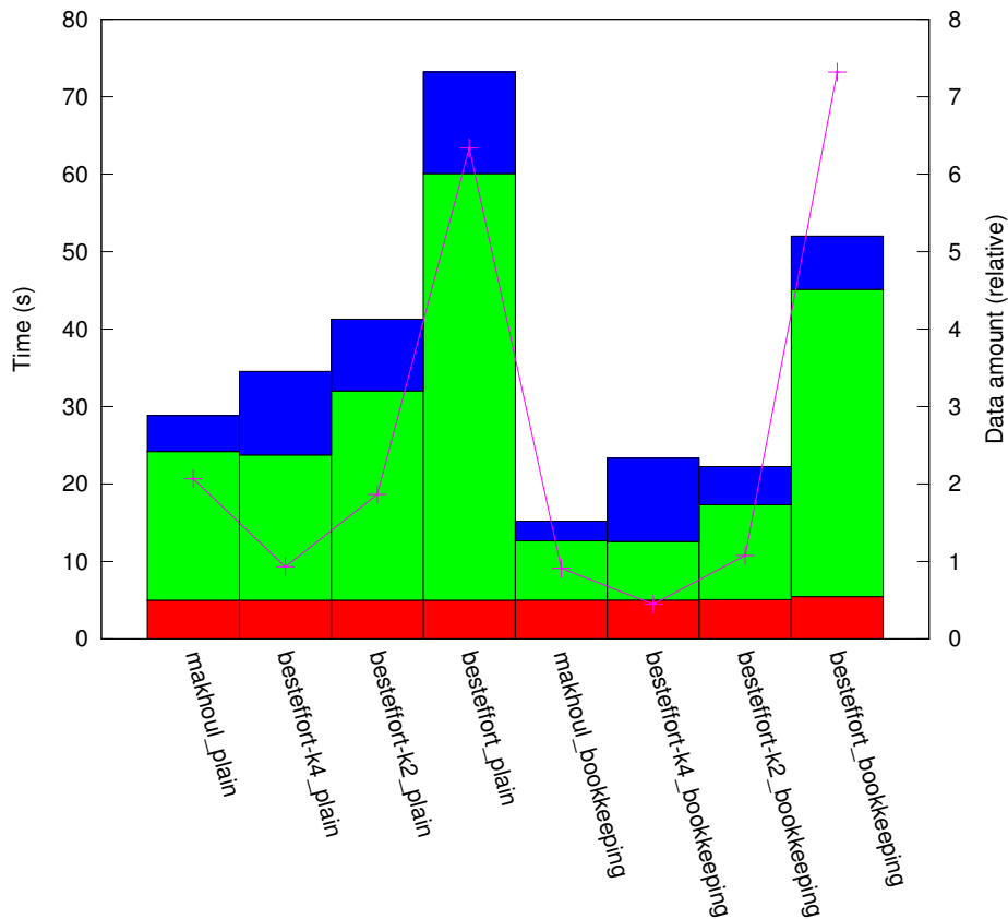
results_IN_10:1/plat_grid256/topo_hcube
